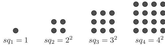
FIGURE 4.8. The square numbers sq_i = i^2 .
