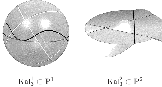
FIGURE 3.3. The Geometry of Kalker's Hypersurfaces. \text{Kal}_3^1 \subset \mathbb{P}^1 consists of two points, one doubled: In the projective view one can see the (black) Fermat cubic x_0^3 + x_1^3 + \frac{1}{4}x_2^3 touching the hyperplane x_0 + x_1 + x_2 \simeq \mathbb{P}^1 in one point and meeting it transversally in another one. To illustrate the construction of the Kalker cubic \text{Kal}_3^2 \subset \mathbb{P}^2 which takes place in \mathbb{P}^3 , we take the affine chart x_3 = 1 . Here one sees the three points in which the hyperplane x_0 + x_1 + x_2 + 1 \simeq \mathbb{P}^2 touches the cubic x_0^3 + x_1^3 + x_2^3 + 1^3 . \text{Kal}_3^2 consists of three lines.
