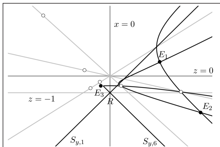
FIGURE 8.3. The 15-nodal plane septic S_{y_{\alpha_R}} = S_{y,1_{\alpha_R}} \cdot S_{y,6_{\alpha_R}} (see (8.11) on page 102); the singularities of the sextic S_{y,6_{\alpha_R}} are marked by large circles: The three exceptional singularities E_1, E_2, E_3 are marked in black, the generic singularities in white. The five left-most nodes are real isolated ones. Only five of the six intersections of the line S_{y,1_{\alpha_R}} and the sextic S_{y,6_{\alpha_R}} are visible because we just show a small part of the whole (x, z) -plane.
