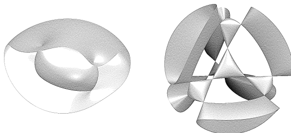
FIGURE 1.3. Fresnel's Wave Surface \text{Fres}_{1, \frac{3}{10}, \frac{1}{2}} of 1819 has 16 nodes only four of which are real. Kummer's tetrahedral-symmetric Surface \text{Ku}_{1,3} of 1864, instead, has 16 real nodes.
